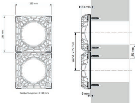
Plastic flange HSI 150-DFK
